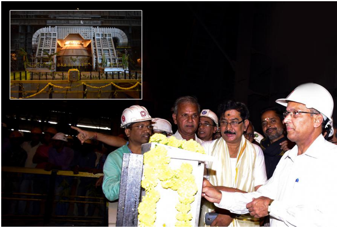
Photo Caption: Sri P Madhusudan, CMD, RINL inaugurating the Converter-3 preheating process in SMS-1 today. (Insert) The revamped Converter-3 in SMS-1
